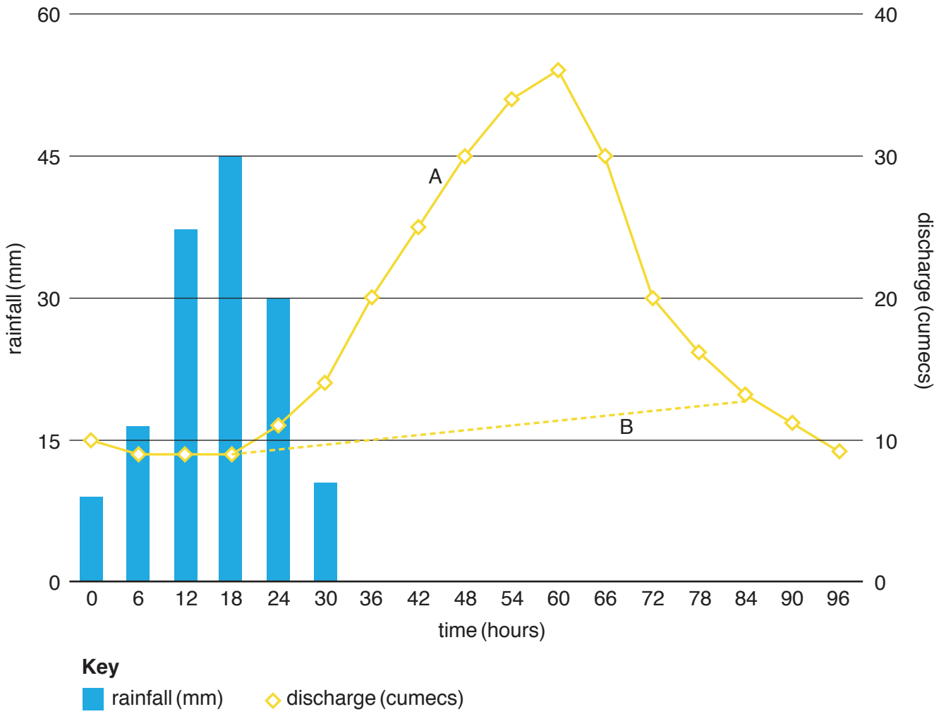
A storm hydrograph
